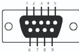
DB9 connector
