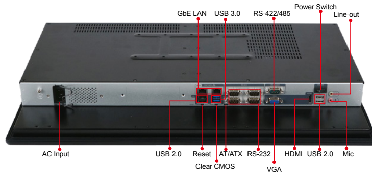
PPC-F24A Fully Integrated I/O
