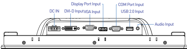
Rear I/O
