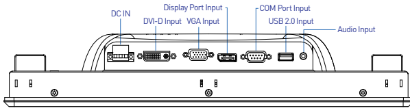
Rear I/O
