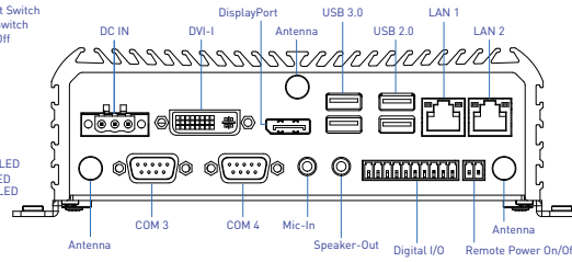
Rear Panel
