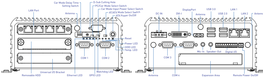
Front Panel
