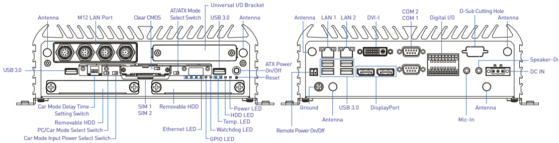
Front Panel
