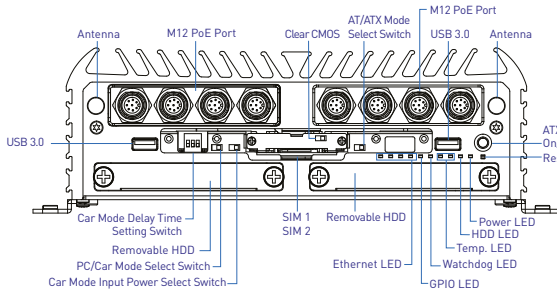
Front Panel
