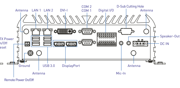
Rear Panel
