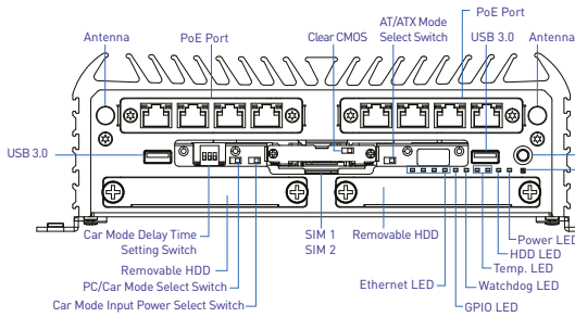
Front Panel
