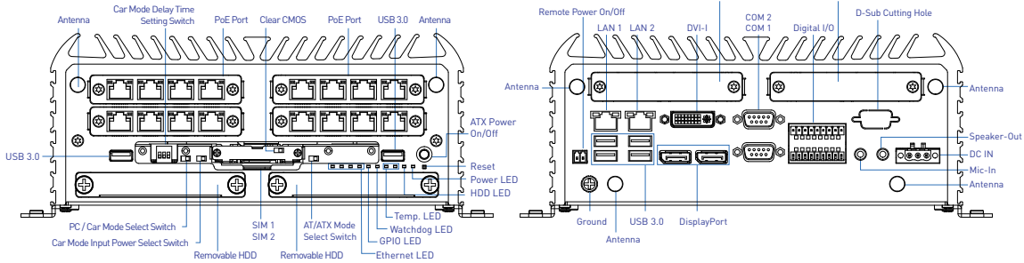
Front Panel
