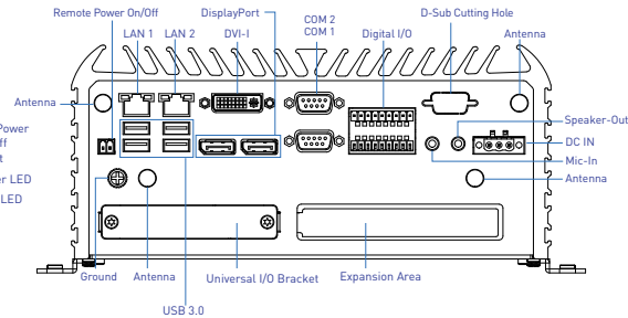
Rear Panel
