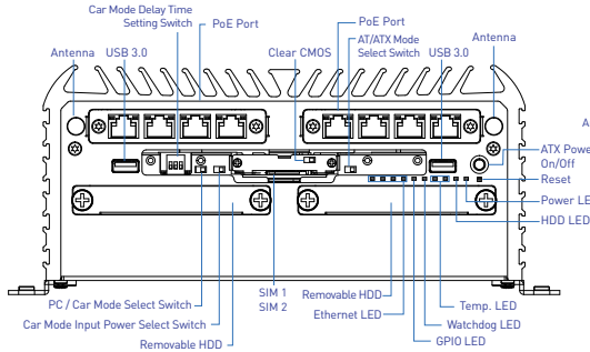
Front Panel
