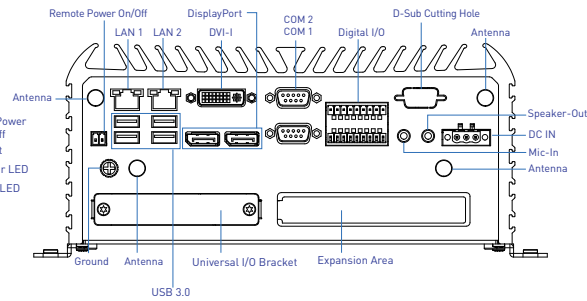
Rear Panel
